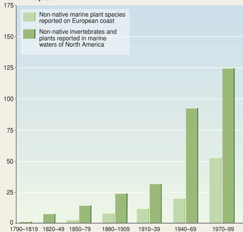
Figure 2.1 GROWTH IN NUMBER OF MARINE SPECIES INTRODUCTIONS
