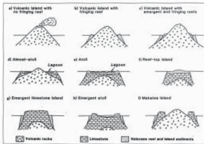
Figure 2: Main types of mid-oceanic islands in the Pacific. (Woodroffe, 1989).
