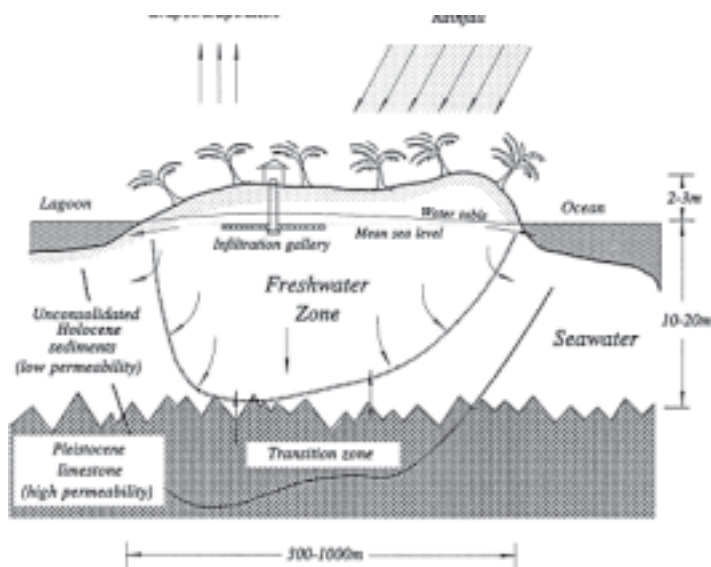
Figure 4: Cross section through a small coral island showing main features of a freshwater lens (exaggerated vertical scale) and location of an infiltration gallery.
