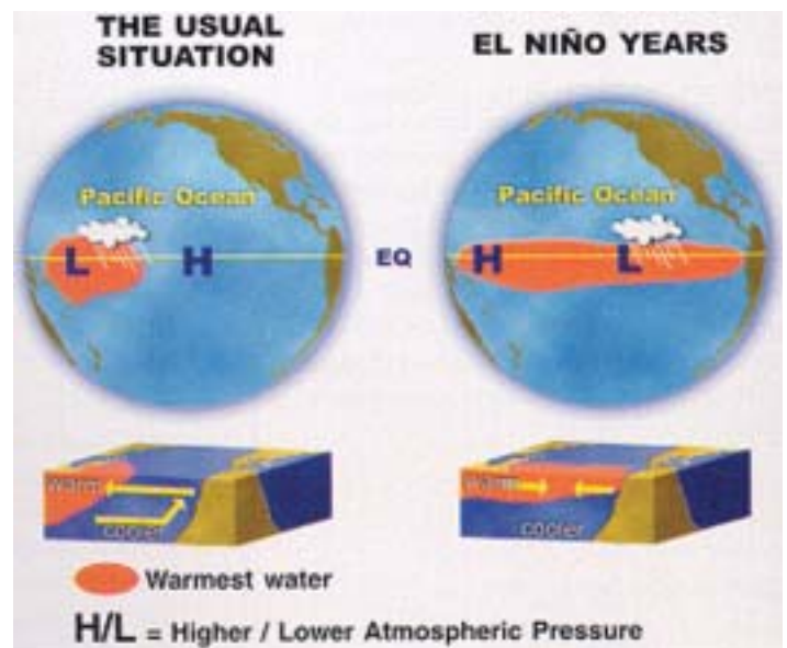
Figure 3: Water and atmosphere processes influence rainfall around the Pacific (modified after WMO brochure).
